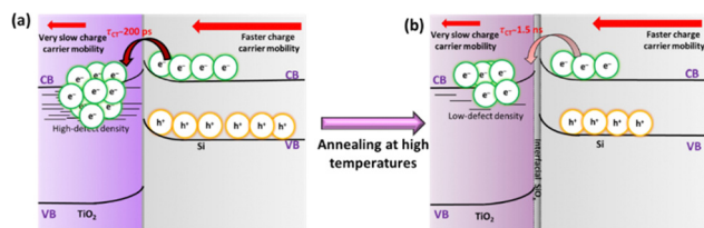
Fig. 6 Schematic of photoinduced interfacial charge transfer in (a) as-dep. TiO 2 /n-Si and (b) 15 min annealed TiO 2 /n-Si samples.
