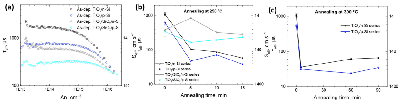
Fig. 2 (a) Injection-level dependent effective lifetimes for Si wafers passivated by 54 nm thin films of (a) as-deposited TiO 2 , (b) annealed TiO 2 films at 250 °C, and (c) annealed TiO 2 films at 300 °C for different durations. The corresponding surface recombination velocities ( S_{\text{eff}} ) are also shown on the right y-axis.
