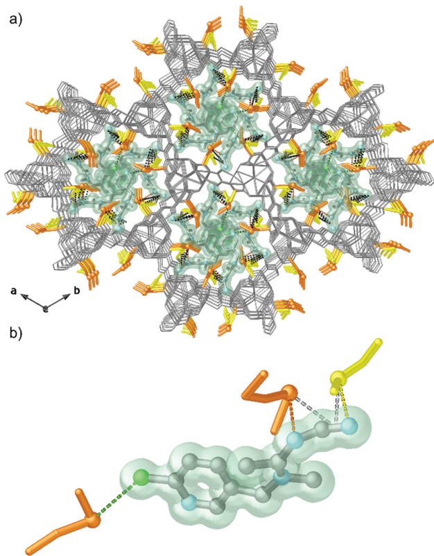
Fig. 9 (a) Perspective view, in the ab plane, of the porous structure of bioMOF Cu 6 SrMet/Mecys with acetamiprid molecules embedded. (b) Detailed view of the captured acetamiprid molecules emphasising the host–guest interactions with thioether groups from L -methionine and S -methyl- L -cysteine amino acids. Guest molecules are represented as green solid surfaces for the sake of clarity. This figure is adapted with permission from ref. 81, copyright ACS 2021.
