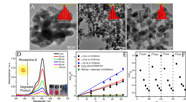
Fig. 5 (A)–(C) TEM images of \alpha -Fe-4, \alpha -Fe-8 and \alpha -Fe 16, respectively (insets show their respective particle size distribution); (D) UV-vis absorption spectra of aq. RhB in the presence of \alpha -Fe-16 under sunlight at different time intervals and corresponding images showing dye degradation; (E) rate of dye degradation and (F) recyclability of \alpha -Fe-16 as a photocatalyst for 4 repeated catalytic cycles. Adopted from ref. 133 with permission. Copyright 2019 The Royal Society of Chemistry.
