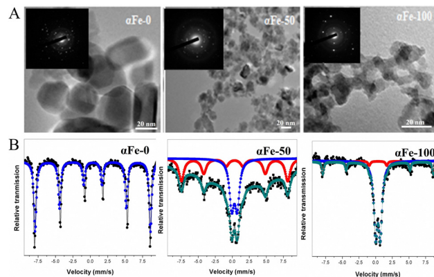
Fig. 4 (A) TEM images; and (B) Mössbauer spectra of \alpha\text{-Fe}_2\text{O}_3 NPs prepared at different IL concentrations in an IL:EG binary mixture. 0, 50 and 100 in (A) and (B) represent the content of IL in the binary mixture, respectively. Adopted from ref. 129 with permission. Copyright 2015 The Royal Society of Chemistry.
