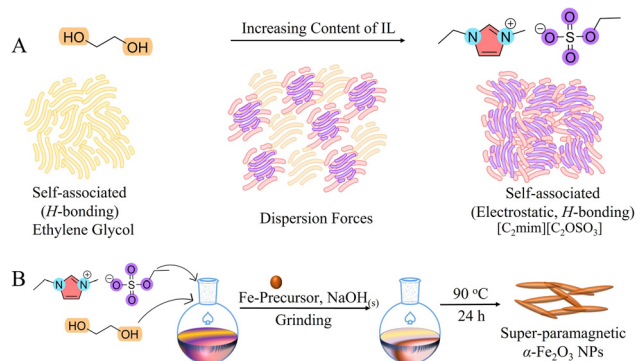
Fig. 3 (A) Interactive forces existing in binary mixtures of IL and EG at varying amounts of ILs; and (B) schematic representation of the procedure of synthesis of \alpha\text{-Fe}_2\text{O}_3 NPs in IL-EG binary mixtures.
