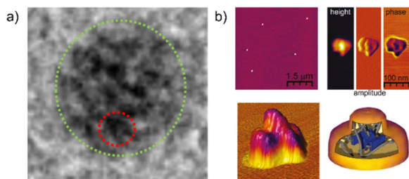
Fig. 11 (a) TEM image of local domains of a Cu-folded SCNP. Reprinted with permission from the American Chemical Society, copyright © 2018 (open access). 75 (b) High resolution AFM image of a SCNP showing a dense core and a less dense shell. Reprinted with permission from the American Chemical Society, copyright © 2010. 29a
