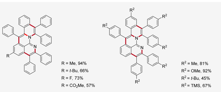
Scheme 4 Electrochemical synthesis of aza-polycyclic aromatic hydrocarbons 14 via rhodaelectro-catalyzed domino C–H annulations.
