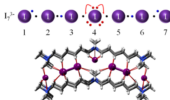
Fig. 7 I_7^{3-} Lewis dot graph and the (symmetrical) anion found in the PEKKEX crystal structure. 49 I–I interatomic distances are 3.388 (1–2 and 6–7), 2.813 (2–3 and 5–6) and 3.427 Å (3–4 and 4–5). Adapted from ref. 4 with permission from RSC, copyright 2021.
