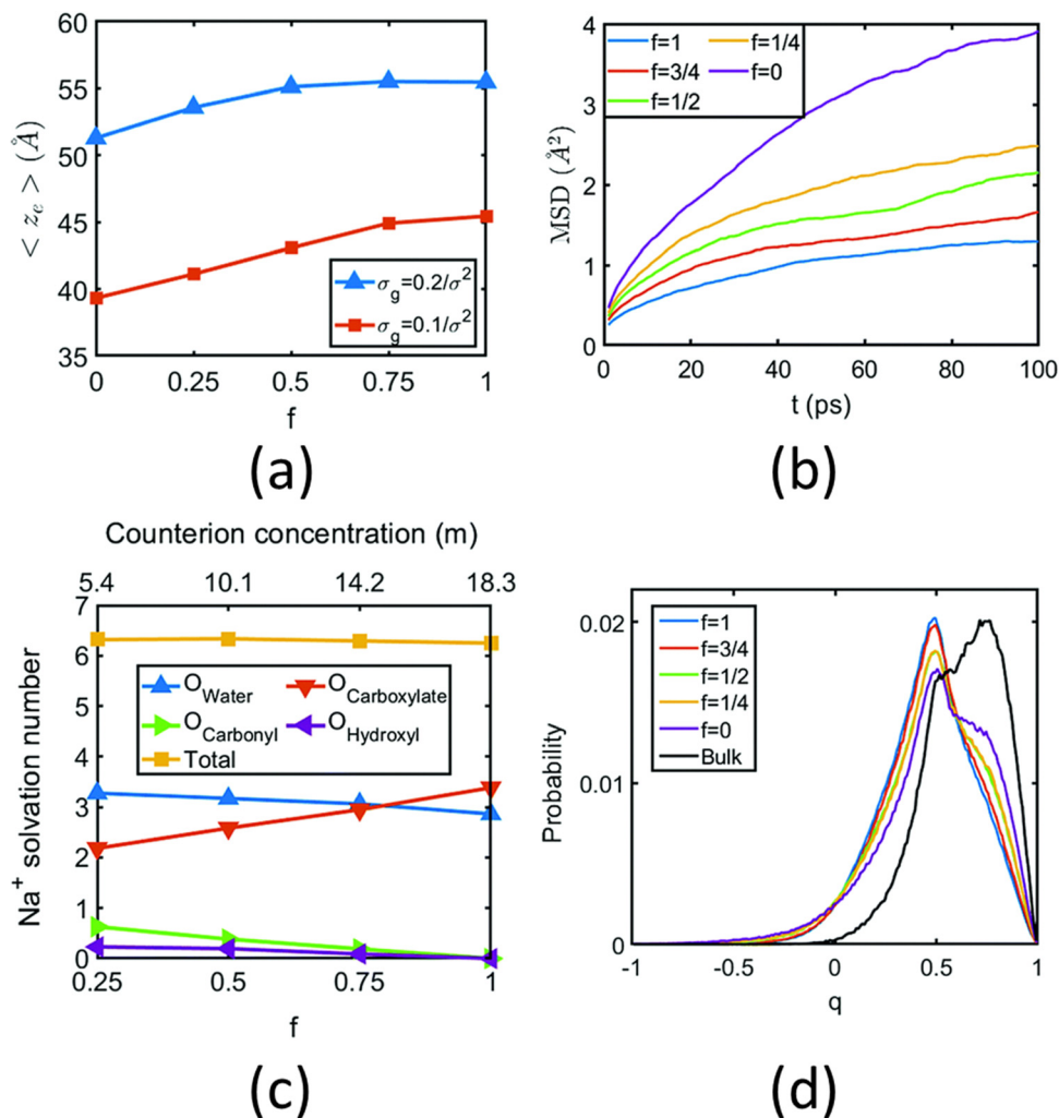
Fig. 11 (a) Variation of the height ( z_c ) of the Na + -counterion-screened PAA PE brushes with degree of ionization ( f ) for two different values of the PE brush grafting density. (b) MSD of the backbone carbon atoms of the PAA PE brushes for different degrees of ionization of the PAA brushes for a grafting density ( \sigma_g ) of 0.1/\sigma^2 chains per nm 2 ( \sigma = 3.5 Å). (c) Change in the composition of the solvation shell of the brush-supported Na + counterions with the degree of ionization of the PAA brushes (for \sigma_g = 0.1/\sigma^2 chains per nm 2 ). (d) Variation in the probability of the tetrahedral order parameter ( q ) of the water molecules with the degree of ionization ( f ) of the PAA brushes (for \sigma_g = 0.1/\sigma^2 chains per nm 2 ). All the parts of the figure have been reproduced from Sachar, H. S.; Pial, T. H.; Chava, B. S.; Das, S., All-atom molecular dynamics simulations of weak polyionic brushes: influence of charge density on the properties of polyelectrolyte chains, brush-supported counterions, and water molecules, Soft Matter , 2020, 16 (33), 7808–7822. Copyright (2020) Royal Society of Chemistry (UK).
