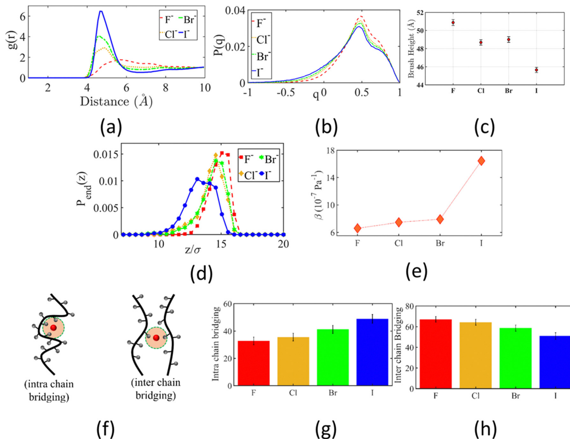
Fig. 24 (a) RDF of \{N(\text{CH}_3)_3\}^+X ( X = \text{I}^-, \text{Br}^-, \text{Cl}^-, \text{and } \text{F}^- ). (b) Probability distribution of the tetrahedral order parameter ( q ) of the solvating water of the \{N(\text{CH}_3)_3\}^+ moiety. (c) Variation of the height of the PMETA + brushes for the cases where the PMETA + brushes are screened by different halide counterions. (d) End chain monomer distributions of the PMETA + brushes. (e) Variation of the compressibility factor of the PMETA + brush system. In (b), (d), and (e), results are shown for the individual cases where the PMETA + brushes are screened by different halide counterions. (f) Schematic of two types of bridging interactions: intrachain bridging and interchain bridging. (g) Percentage of intrachain bridging undergone by the monomers of the PMETA + chains screened by different halide counterions. (h) Percentage of interchain bridging undergone by the monomers of the PMETA + chains screened by different halide counterions. All the parts of the figure have been reprinted with permission from Ishraaq, R.; Das, S., All-Atom molecular dynamics simulations of cationic polyelectrolyte brushes in the presence of halide counterions, Macromolecules , 2024, 57 (7), 3037–3046. Copyright (2024) American Chemical Society.
