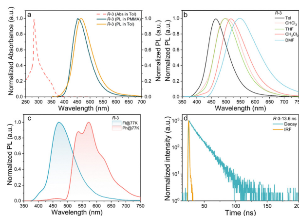
Fig. 3 Photophysical properties of R-3 . (a) Normalised UV absorption (dashed line) and PL spectra in toluene solution ( 10^{-5} M) and doped in PMMA film ( \lambda_{\text{ex}} = 350 nm); (b) PL spectra in different solvents at room temperature; (c) low temperature fluorescence and phosphorescence (delayed 2 ms) spectra in toluene solution; (d) time-resolved emission of R-3 in toluene solution ( 10^{-5} M) ( \lambda_{\text{ex}} = 350 nm).
