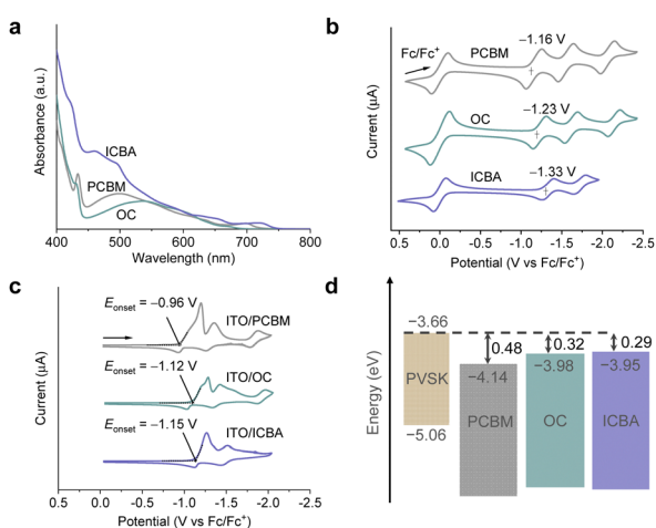
Fig. 2 (a) UV-vis absorption spectra of PCBM, OC, and ICBA ( 50\text{ }\mu\text{M} ). (b) Cyclic voltammograms (CV) of PCBM, OC, and ICBA in ODCB ( 1.0\text{ mM} ). (c) CV for spin-coated PCBM, OC, and ICBA films in acetonitrile. (d) Energy level diagrams of \text{PEA}_{0.15}\text{FA}_{0.85}\text{SnI}_3 and PCBM, OC, and ICBA films. PVSK denotes \text{PEA}_{0.15}\text{FA}_{0.85}\text{SnI}_3 perovskites.
