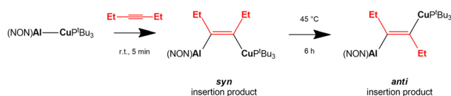
Scheme 8 Experimental insertion of internal 3-hexyne in the Cu–Al bond of the [{}^t\text{Bu}_3\text{PCuAl}(\text{NON})] complex. 68
