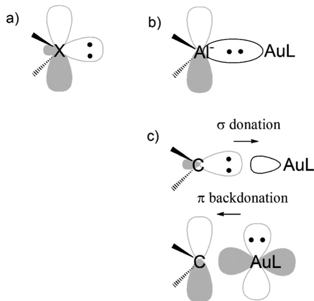
Scheme 3 Schematic representation of the (a) isolobal analogy between singlet carbenes and aluminyls: lone pair and vacant 2p/3p orbitals on the X = C and X = \text{Al}^- sites of carbenes and aluminyls, respectively; (b) electron-sharing bond in a gold–aluminyl complex; (c) Dewar–Chatt–Duncanson bonding model in a gold–carbene analogue (dative bond).
