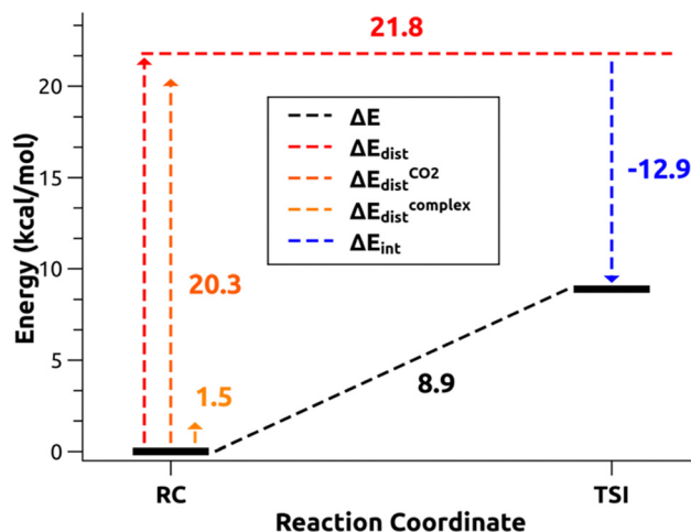
Fig. 11 Activation strain model (ASM) decomposition of the electronic energy activation barrier between RC and TSI for the reaction of [^t\text{Bu}_3\text{PAuAl}(\text{NON})] complex and carbon dioxide. Adapted with permission from ref. 26 Copyright 2021, American Chemical Society.
