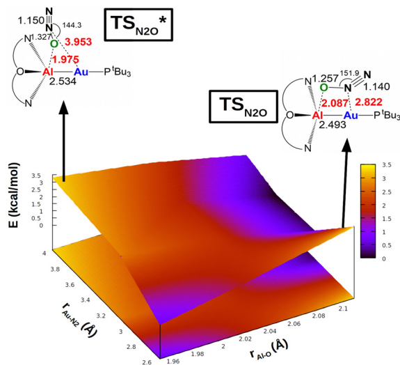
Fig. 6 Potential energy surface (PES) in the region neighbouring the transition state TS for the reaction of complex [{}^t\text{Bu}_3\text{PAuAl}(\text{NON})] with N_2O . Insets: Position on the PES and schematic structure of TS and \text{TS}^* . Energy has been shifted in each case according to the minimum energy structure. Reproduced with permission from ref. 63 Copyright 2023, Wiley-VCH GmbH.
