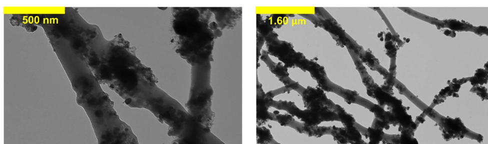
Fig. 2 TEM images of CNF/TiO 2 composites with 50 wt% TiO 2 .
