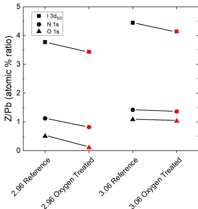
Fig. 4 The atomic percentage ratios of iodine, nitrogen, and oxygen relative to the Pb 4f_{7/2} doublet for an understoichiometric and overstoichiometric sample. All ratios decrease upon photooxygen treatment.
