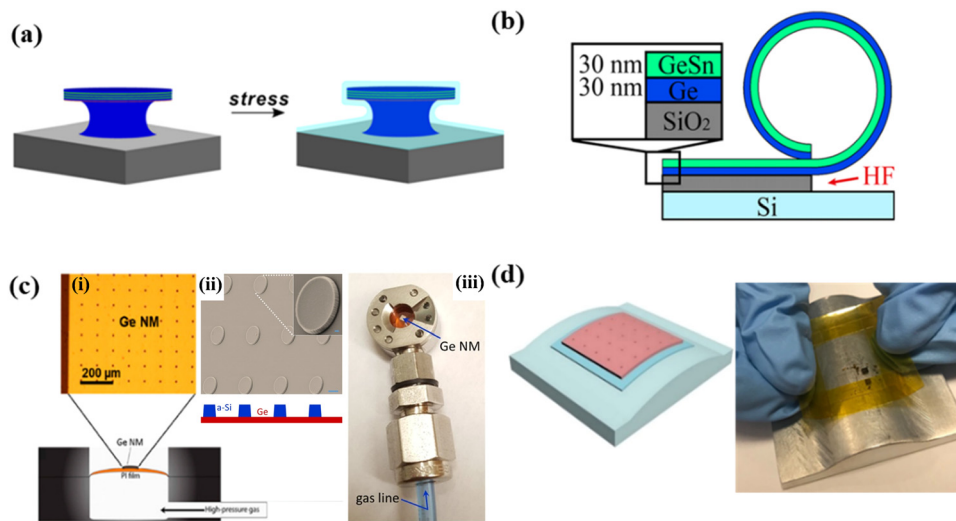
Fig. 4 Various strain-engineering strategies for GeSn NMs: (a) Tensile strained GeSn microdisk using high-stress \text{Si}_3\text{N}_4 stressor layer. 58 Reprinted with permission from ref. 58. Copyright 2016, American Chemical Society. (b) A schematic diagram describing the rolling up procedure for the GeSn/Ge bilayer. 59 Reproduced with permission from ref. 59. Copyright 2018, IOP Publishing. (c) (i) Schematic illustration of the experimental setup for biaxial tensile strained Ge NMs, 60 (ii) SEM image with a schematic of a Ge NM coated with an a-Si pillar array, and a photograph of the pressure cell loaded with a Ge NM. 61 Reproduced with permission from ref. 60 and 61. Copyright 2018, 2021, MDPI, American Chemical Society. (d) Schematic structure and optical image of flexible GeSn NMs where uniaxial strains are introduced by placing conformally on bending fixtures. 62 Reproduced with permission from ref. 62. Copyright 2021, IOP Publishing.
