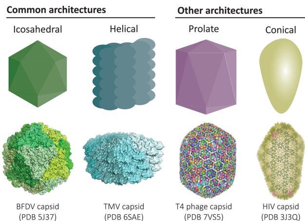
Fig. 1 Common architectures found in protein cages and virus-like particles. Icosahedral and helical symmetries are most common, 12,13 while there also exists elongated prolate structures and conical assemblies, amongst other less common architectures. 14,15
