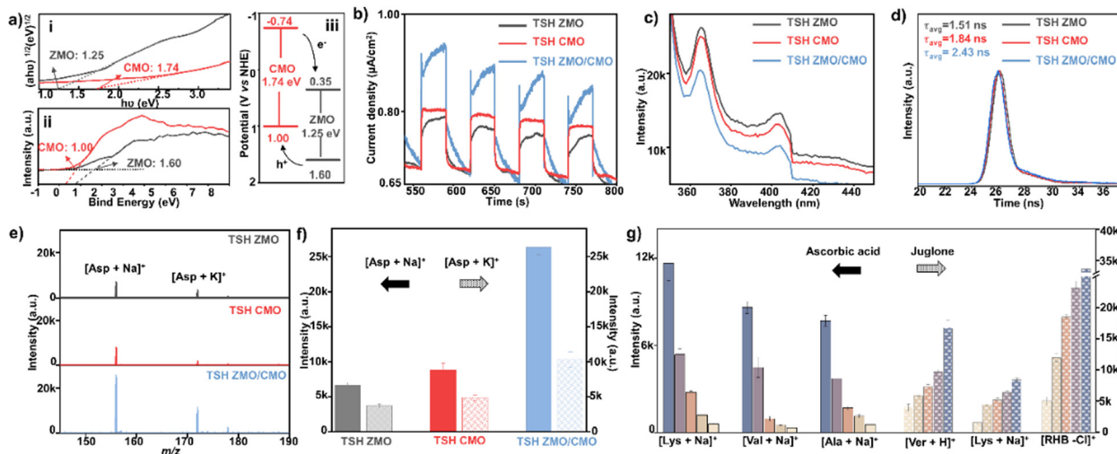
Fig. 4 The heterojunction effect of TSH ZMO/CMO on LDI-MS detection of metabolites. (a) (i) The corresponding Tauc plots from UV-Vis diffuse reflectance spectra and (ii) the E_g from the VB X-ray photoelectron spectroscopy spectra and (iii) schematic diagram of the charge separation and transfer in the TSH ZMO/CMO composites. (b) The relative peak intensities of photocurrent–time curves, (c) PL spectrum, and (d) TRPL spectra based on TSH ZMO, TSH CMO, and TSH ZMO/CMO ( P < 0.05 ). (e) The typical LDI-MS spectra of 0.1 mg mL -1 of Asp using TSH ZMO, TSH CMO, and TSH ZMO/CMO as the matrices. (f) Mean intensities of Na + and K + adducted peaks for 0.1 mg mL -1 of Asp in 3 experiments using TSH ZMO, TSH CMO, and TSH ZMO/CMO as the matrices. (g) LDI-MS results of Lys, Val, and Ala in ascorbic acid (AA) and Ver, Lys, and RHB in juglone using TSH ZMO/CMO as the matrix (from blue to light yellow: the concentration of AA/juglone increases gradually).
