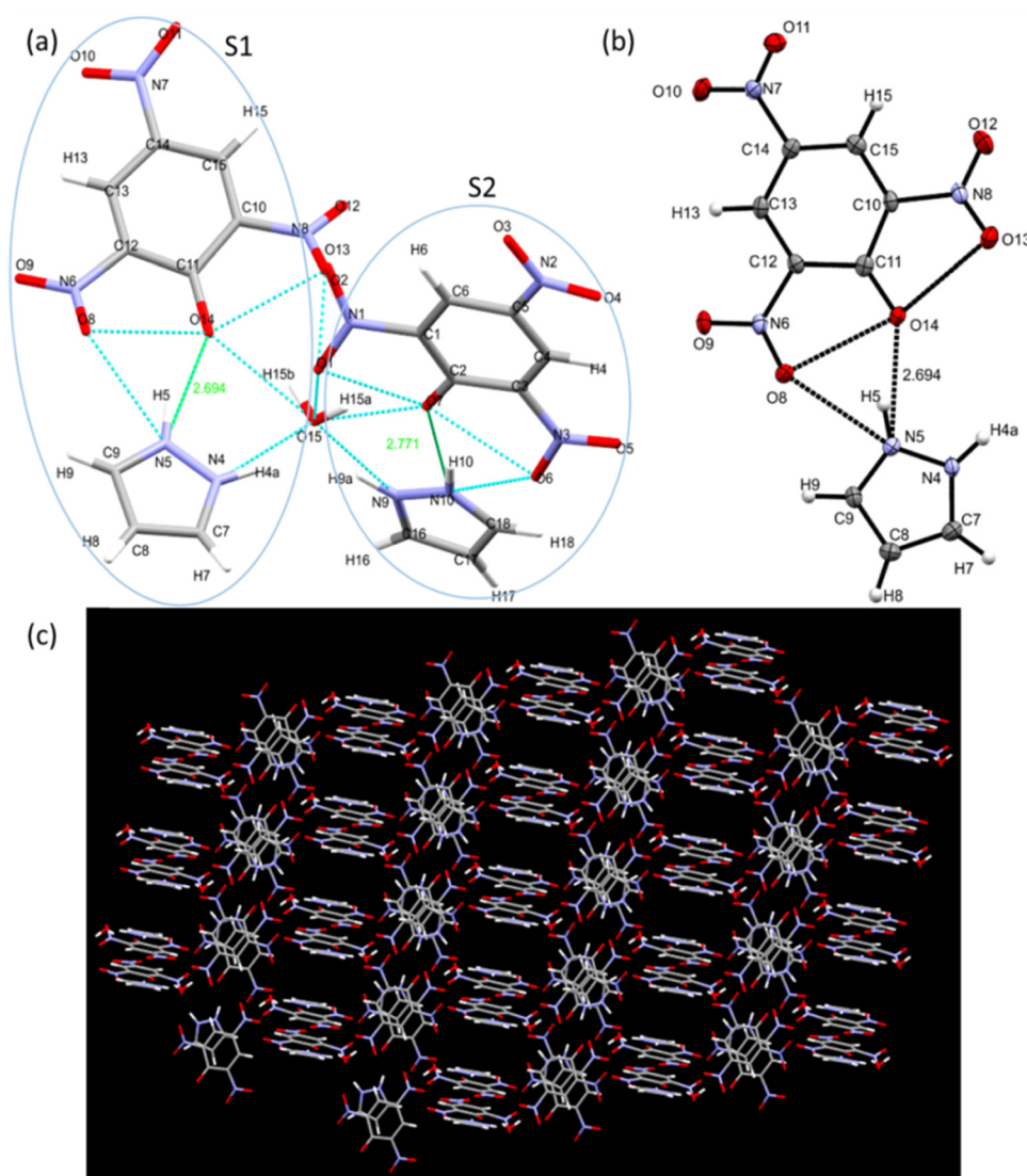
Fig. 15 (a) Structure showing twin sisters S1 and S2 bonded with a water molecule, (b) an orped view showing interaction between the donor and acceptor moieties, and (c) crystal packing showing the hydrogen bonding network.
