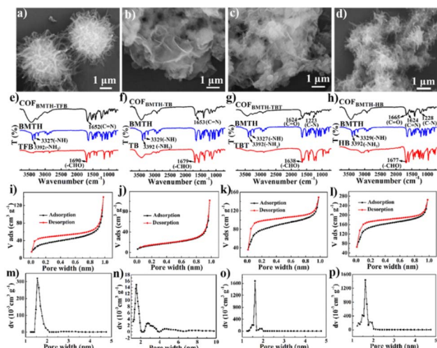
Fig. 1 SEM images (a–d), FTIR spectra (e–h), N 2 adsorption/desorption isotherms (i–l) and the pore size distribution (m–p) of COF BMTH-TFB (a, e, i and m), COF BMTH-TB (b, f, j and n), COF BMTH-TBT (c, g, k and o) and COF BMTH-HB (d, h, l and p), respectively.
