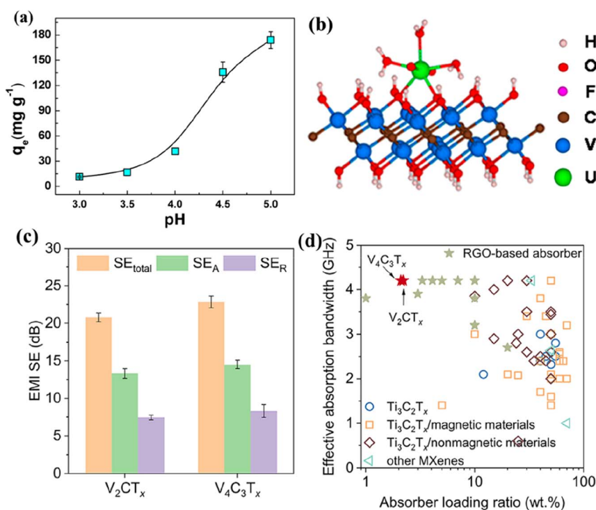
Fig. 9 (a) Adsorption of uranium on \text{V}_2\text{CT}_x as a function of pH and the adsorption configuration (b). Reproduced with permission from ref. 158 copyright 2016, American Chemical Society. (c) The average EMI shielding effectiveness of \text{V}_2\text{CT}_x and \text{V}_4\text{C}_3\text{T}_x coatings on glass substrates and (d) EM wave absorption performance of \text{V}_{n+1}\text{C}_n\text{T}_x/\text{PU} composites compared with reported \text{Ti}_3\text{C}_2\text{T}_x -based composites and other materials from ref. 159.
