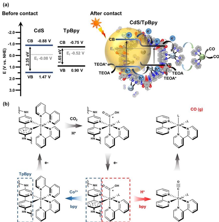
Scheme 1 (a) Schematic representation of the reaction mechanism of photocatalytic CO _2 reduction using CdS/TpBpy as the catalyst, [Co(bpy) _3 ] ^{2+} as the cocatalyst, and TEOA as the hole scavenger, under sunlight irradiation. (b) Proposed mechanism of CO _2 photoreduction to CO by [Co(bpy) _3 ] ^{2+} .
