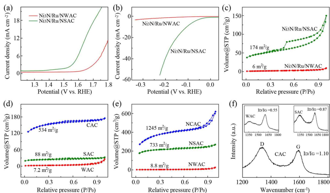
Fig. 4 (a, b) LSV curves of \text{Ni}_3\text{N}/\text{Ru}/\text{NWAC} and \text{Ni}_3\text{N}/\text{Ru}/\text{NSAC} composites for the OER and HER, respectively. Scan rate: 5 mV \text{s}^{-1} . (c–e) Nitrogen adsorption–desorption isotherms. (c) \text{Ni}_3\text{N}/\text{Ru}/\text{NWAC} and \text{Ni}_3\text{N}/\text{Ru}/\text{NSAC} composites. (d) WACs, SACs and CACs. (e) NWACs, NSACs and NCACs. (f) Raman spectra of WACs, SACs and CACs.
