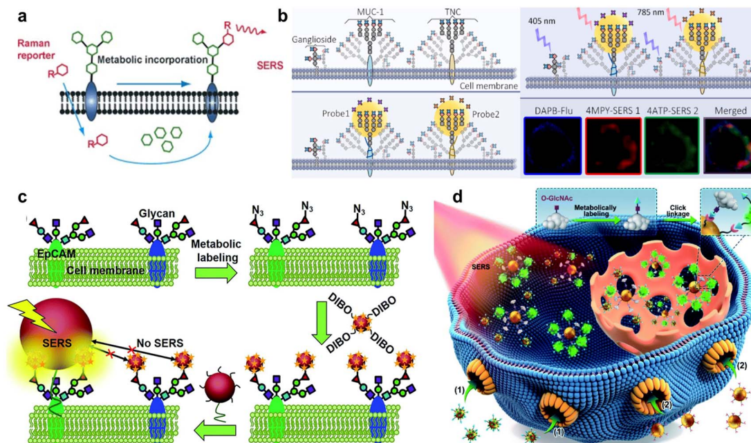
Fig. 9 (a) Bioorthogonal Raman reporter strategy for SERS detection of glycans on live cells. Reprinted with permission from ref. 86. Copyright 2013, Wiley-VCH. (b) Classification process for the profiling of cell-surface SA subgroups. Reprinted with permission from ref. 94. Copyright 2021, Elsevier B.V. (c) Zone-controllable SERS effect for imaging of protein-specific glycans on the cell surface. Reprinted with permission from ref. 95. Copyright 2016, The Royal Society of Chemistry. (d) Quantitative SERS imaging strategy for O-GlcNAcylation mapping of single living cells. Reprinted with permission from ref. 97. Copyright 2022, The Royal Society of Chemistry.
