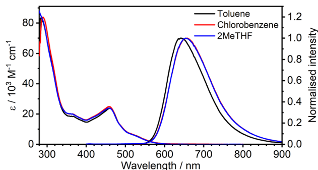
Fig. 2 Absorption and photoluminescence ( \lambda_{\text{ex}} = 365 \text{ nm} ) spectra of 1 in the three solvents indicated at a concentration of approximately 10^{-5} \text{ M} .
