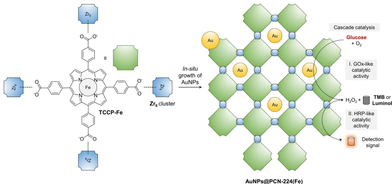
Fig. 1 Schematic illustration of the construction of a bifunctional nanozyme, \text{AuNPs@PCN-224(Fe)} , through the in situ growth of AuNPs inside a MOF formed by the coordination between \text{Fe(II)} meso-tetra(4-carboxyphenyl)porphine (TCPP-Fe) and zirconyl chloride octahydrate ( \text{Zr}_6 cluster) for the cascade catalysis of D-glucose to produce colorimetric and chemiluminescent signals. TMB = 3,3',5,5'-tetramethylbenzidine.
