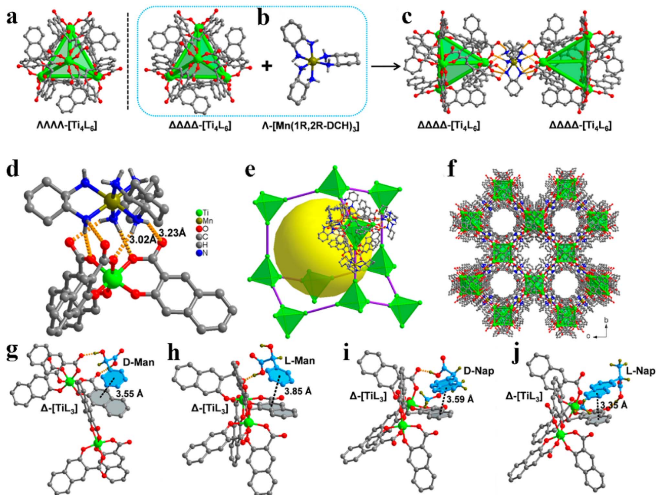
Fig. 23 (a) Molecular structures of the \Delta\Delta\Delta\Delta -[Ti 4 L 6 ] and \Lambda\Lambda\Lambda\Lambda -[Ti 4 L 6 ] enantiomers. (b) \Lambda -[Mn(1R,2R-DCH) 3 ] unit in PTC-108( \Delta ). (c) Two adjacent \Delta\Delta\Delta\Delta -[Ti 4 L 6 ] cages linked by one \Lambda -[Mn(1R,2R-DCH) 3 ] unit. (d) N–H...O H-bonds in PTC-108( \Delta ). (e and f) Diamondoid cage and 3D framework of PTC-108( \Delta ). (Ti, green; Mn, olive; O, red; N, blue; C, gray). (g–j) Illustration of the proposed recognition models of the PTC-108( \Delta ) cage towards enantiomers. 70 Reproduced with permission from ref. 70. Copyright 2018, the American Chemical Society.
