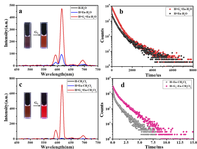
Fig. 4 Luminescent emission spectra of (a) H (black line), H/Eu^{3+} (blue line), and H/Eu^{3+}/G_1 (red line), and time-resolved photoluminescence decay curves of (b) H/Eu^{3+} (black line) and H/Eu^{3+}/G_1 (red line) in aqueous solution at 298 K. (c) Corresponding emission and (d) time-resolved photoluminescence decay curves in CH_2Cl_2 solution ( [H] = 2.0 \times 10^{-5} \text{ M} ) at 298 K.
