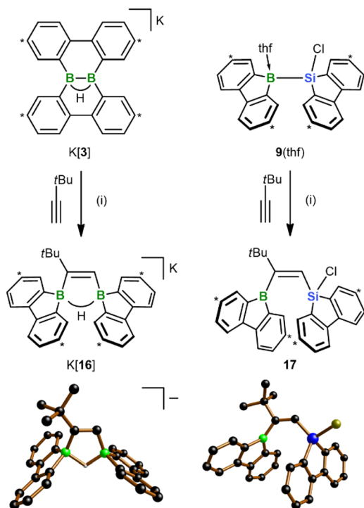
Scheme 6 Diboration and silaboration of t\text{BuC}\equiv\text{CH} , starting from K[3] or the chlorosilane 9(thf) and furnishing K[16] and 17 , respectively. Carbon atoms marked with “*” bear t Bu groups. In the crystal-structure plots, the [\text{K}(\text{thf})_2]^+ counter cation of [\mathbf{16}]^- , C-bonded H atoms, and Ar-bonded t Bu groups are omitted for clarity; H: gray, B: green, C: black, Si: blue, Cl: yellow. (i) THF- d_8 , RT, quant. conv. by NMR.
