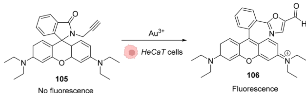
Fig. 35 Generation of fluorescence inside HeCaT cells by the generation of 106 after incubation with Au^{III} . 84,85
