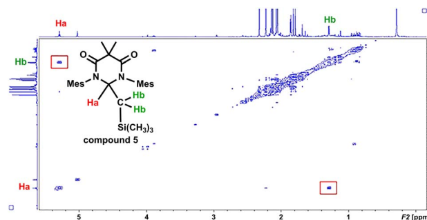
Fig. 8 ^1\text{H} – ^1\text{H} correlation spectrum (COSY) of compound 5 from 0 – 5.6 \text{ ppm} .
