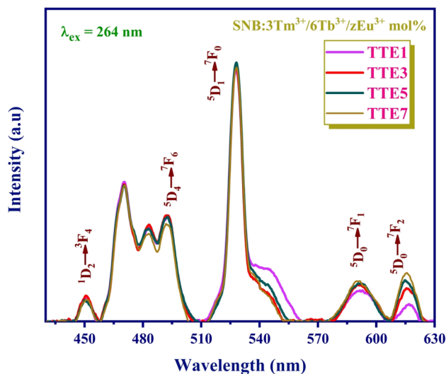
Fig. 9 PL spectra of SNB:3 mol% \text{Tm}^{3+} /6 mol% \text{Tb}^{3+} /z mol% \text{Eu}^{3+} phosphors under 264 nm excitation wavelength.
