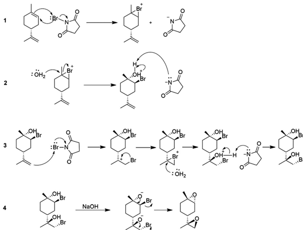
Scheme 27 NBS-mediated stereoselective epoxidation of ( R )-(+)-limonene, reaction mechanism.
