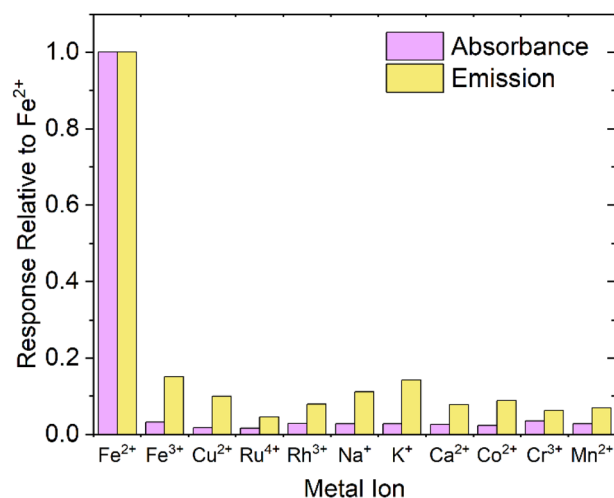
Fig. 6 The response of other common metal ions ( \text{Fe}^{3+} , \text{Cu}^{2+} , \text{Ru}^{4+} , \text{Rh}^{3+} , \text{Na}^{+} , \text{K}^{+} , \text{Ca}^{2+} , \text{Co}^{2+} , \text{Cr}^{3+} , \text{Mn}^{2+} ), with the ferrozine assay (absorbance) and ferrozine-UCNP assay (emission, using PAA-capped PTIR545 UCNPs), relative to the response produced by \text{Fe}^{2+} .
