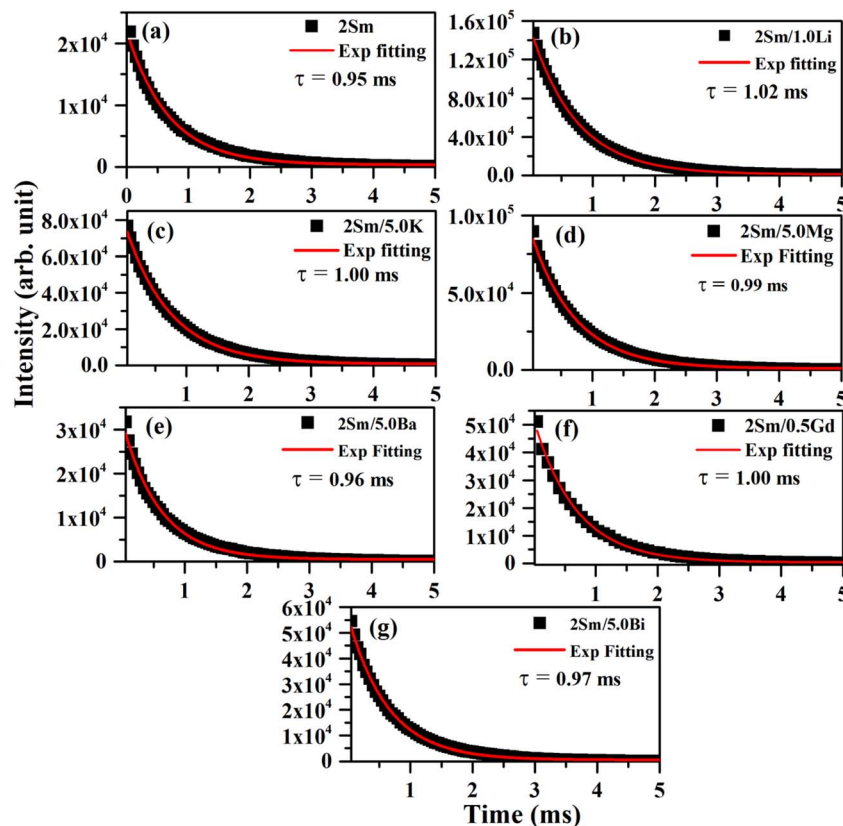
Fig. 10 Decay curves for the ^4G_{5/2} level of \text{Sm}^{3+} ions under \lambda_{\text{ex}} = 407 nm and \lambda_{\text{em}} = 599 nm for (a) \text{CaTiO}_3:2\text{Sm}^{3+} , (b) \text{CaTiO}_3:2\text{Sm}^{3+}/1.0\text{Li}^+ , (c) \text{CaTiO}_3:2\text{Sm}^{3+}/5.0\text{K}^+ , (d) \text{CaTiO}_3:2\text{Sm}^{3+}/5.0\text{Mg}^{2+} , (e) \text{CaTiO}_3:2\text{Sm}^{3+}/5.0\text{Ba}^{2+} , (f) \text{CaTiO}_3:2\text{Sm}^{3+}/0.5\text{Gd}^{3+} and (g) \text{CaTiO}_3:2\text{Sm}^{3+}/5.0\text{Bi}^{3+} phosphors.
