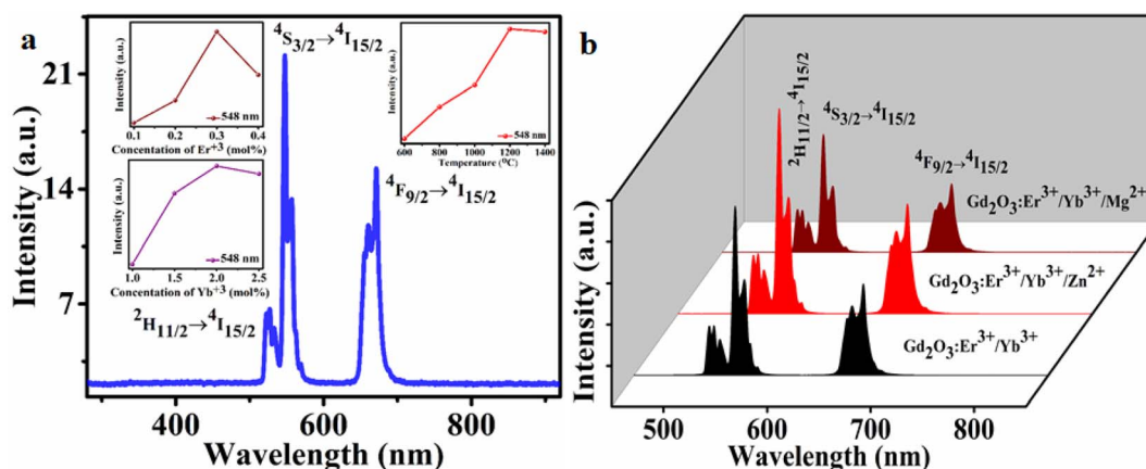
Fig. 4 (a) Whole recorded UC emission spectrum in 280–920 nm range, inset up (left) shows the emission intensity of the band 4\text{S}_{3/2} \rightarrow 4\text{I}_{15/2} at 548 nm with the concentration of \text{Er}^{3+} ions, inset (down) shows the intensity with the concentration of \text{Yb}^{3+} ions, and inset up (right) shows the intensity with annealed temperature, (b) the UC intensity for without tri-depend and with tri-doped atom (8 mol%) of \text{Zn}^{2+} and \text{Mg}^{2+} respectively. For UC measurement excitation source: 980 nm NIR-laser.
