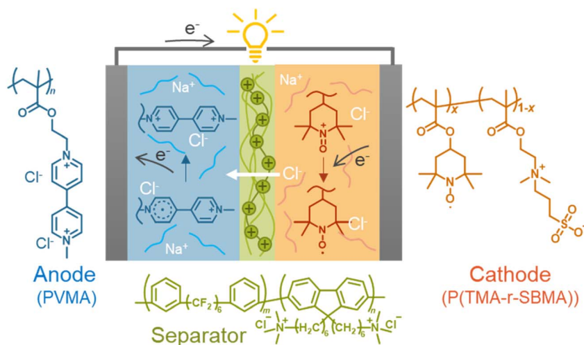
Fig. 1 Configuration of the rechargeable cell examined in this study.
