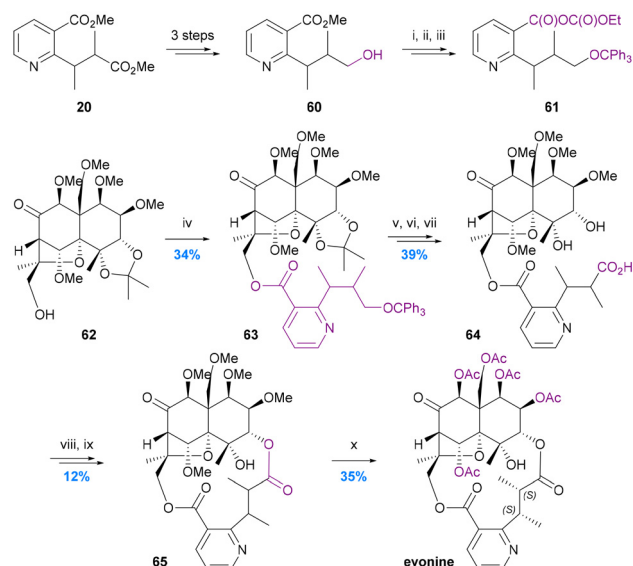
Chart 11 Yamada's resynthesis of evonine. Yamada et al. 1975, 62 (i) Ph 3 CCl–Py, 60 °C; (ii) 10% KOH–MeOH, 70 °C; (iii) ethyl chloroformate, Et 3 N, DME, RT; (iv) crude 61 , DMAP, Et 3 N, DME, 90 °C; (v) 80% AcOH, 50 °C; (vi) CrO 3 –Py, 65 °C; (vii) 50% AcOH, 85 °C; (viii) CH 2 N 2 ; (ix) NaH, DMF, RT; (x) BCl 3 –CH 2 Cl 2 , RT, and then AcO 2 –Py, 70 °C.
