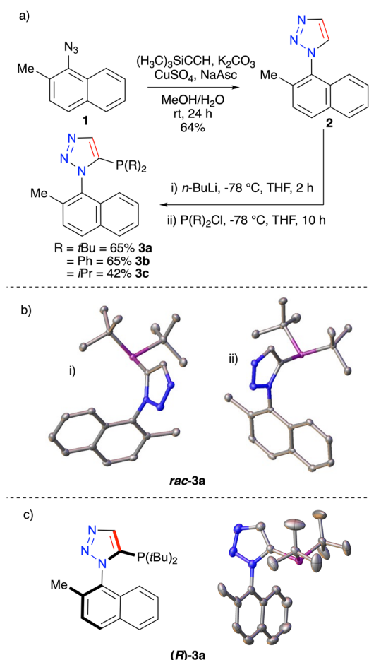
Fig. 2 (a) Synthesis of 1,2,3-triazole phosphines (b) molecules from the crystal structure of \text{rac-3a} with ellipsoids drawn at the 50% probability level. Symmetry codes used to generate the equivalent atoms: (i) x, y, z , (ii) 1 - x, 1 - y, 1 - z . Hydrogen atoms omitted for clarity (c) single-crystal X-ray diffraction structure of (R)\text{-3a} . Ellipsoids are drawn at the 50% probability level. Hydrogen atoms omitted for clarity.
