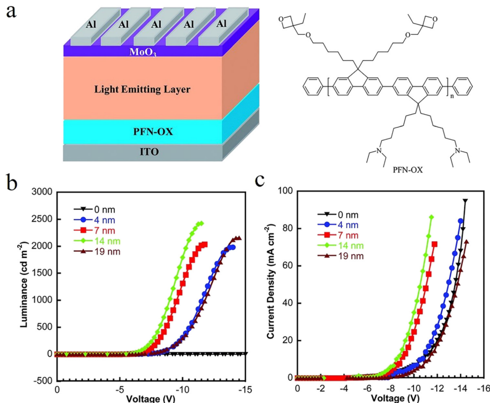
Fig. 3 (a) The device configuration of the inverted OLED and the chemical structures of PFN-OX and light emitting layer materials used in this study. (b) L-V and (c) J-V curves of blue light devices with different thicknesses of the PFN-OX interlayer. 91 Copyright 2014 The Royal Society of Chemistry.
