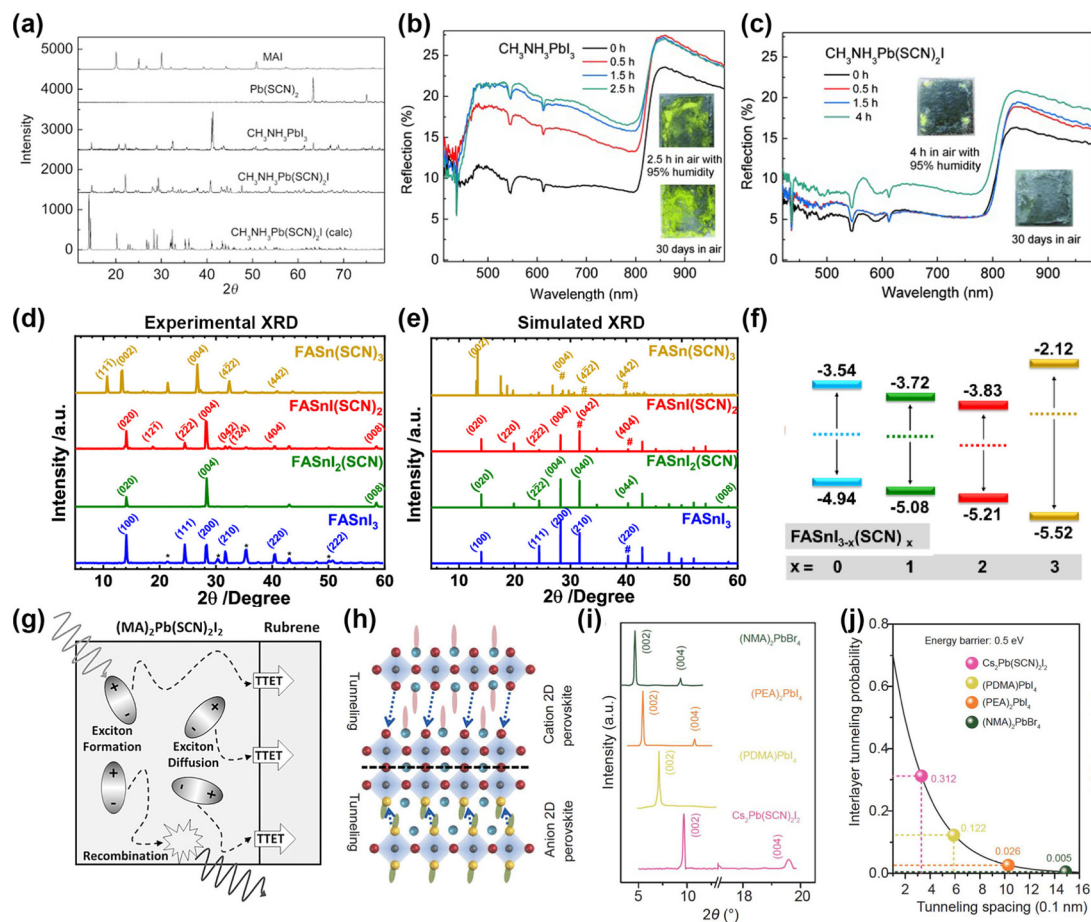
Fig. 3 (a) XRD patterns of \text{MAPbI}_3 and \text{MAPbI}(\text{SCN})_2 perovskite films. (b and c) Reflection spectrum with stability tests of \text{MAPbI}_3 and \text{MAPbI}(\text{SCN})_2 in the air with 95% humidity. Reproduced with permission. 48 Copyright 2015, Wiley-VCH Publications. (d and e) Experimental and simulated XRD patterns of \text{FASn}_{3-x}(\text{SCN})_x perovskite films. (f) Energy level diagrams of \text{FASn}_{3-x}(\text{SCN})_x perovskites. Reproduced with permission. 52 Copyright 2020, American Chemical Society. (g) Exciton diffusion and triplet-triplet energy transfer at the 2D perovskites/rubrene interface. Reproduced with permission. 55 Copyright 2017, Wiley-VCH Publication. (h) The lattice structure of \text{Cs}_2\text{PbI}_2(\text{SCN})_2 perovskites. (i) XRD patterns of four types of 2D perovskites. (j) Relationship between charge channeling probability and interlayer spacing. Reproduced with permission. 57 Copyright 2021, Springer Nature.
