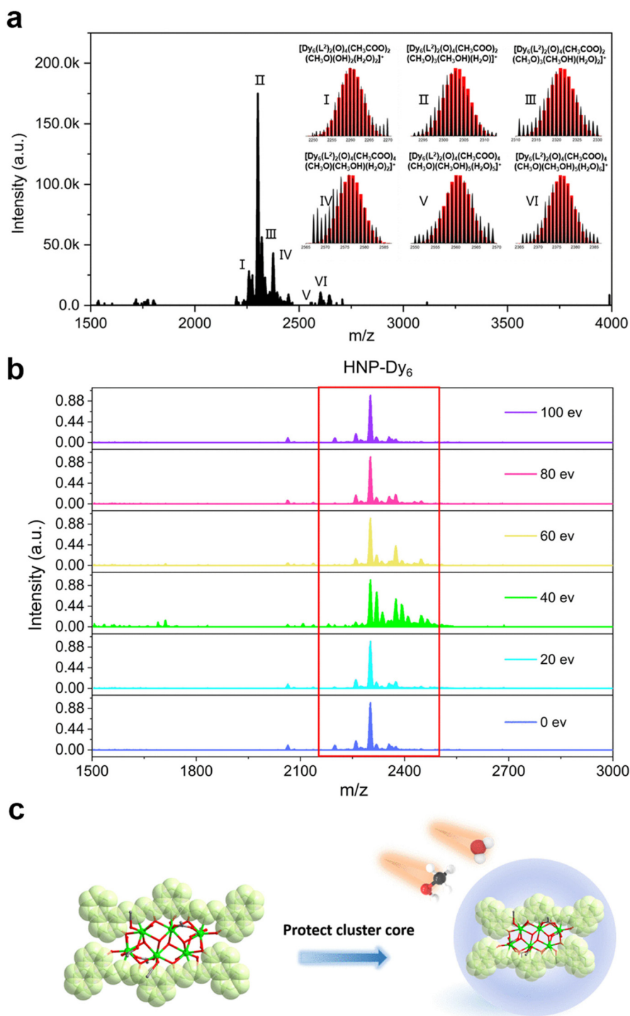
Fig. 4 (a) HRESI-MS spectrum of HNP- \text{Dy}_6 dissolved in DMF in the positive-ion mode, (b) HRESI-MS spectrum of HNP- \text{Dy}_6 dissolved in DMF under different ion-source voltages (in-source CID), and (c) schematic of the chelating ligands effectively protecting the cluster core.
