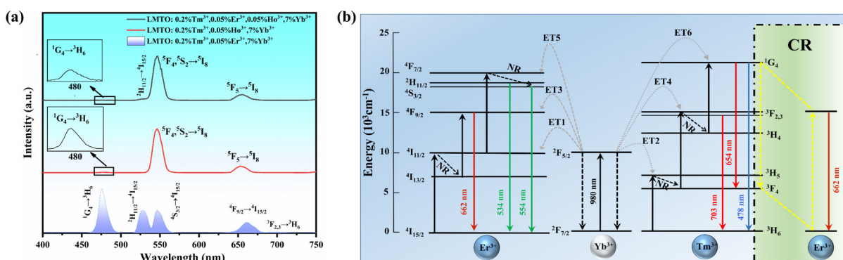
Fig. 6 Mode IV (a) Emission spectra of LMTO:0.2%Tm 3+ ,0.05%Er 3+ ,0.05%Ho 3+ ,7%Yb 3+ ; LMTO:0.2%Tm 3+ ,0.05%Ho 3+ ,7%Yb 3+ and LMTO:0.2%Tm 3+ ,0.05%Er 3+ ,7%Yb 3+ phosphors. (b) The ET processes in Er 3+ , Tm 3+ -Yb 3+ co-doped LMTO system.
