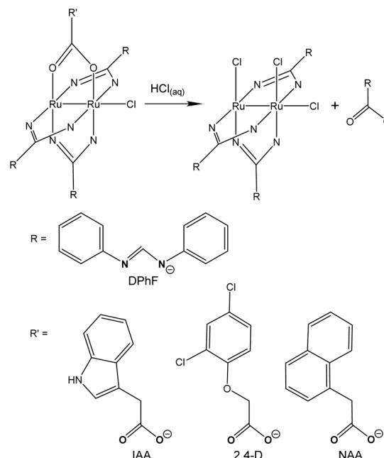
Fig. 4 The pH-dependent release of the auxin ligand ( \mu -R'COO, R' is either indole-3-acetate (IAA), 2,4-dichlorophenoxyacetate (2,4-D), or 1-naphthaleneacetate (NAA) from the Ru(II)Ru(III) complexes of N,N' -diphenylformamidinates (RCNN).
