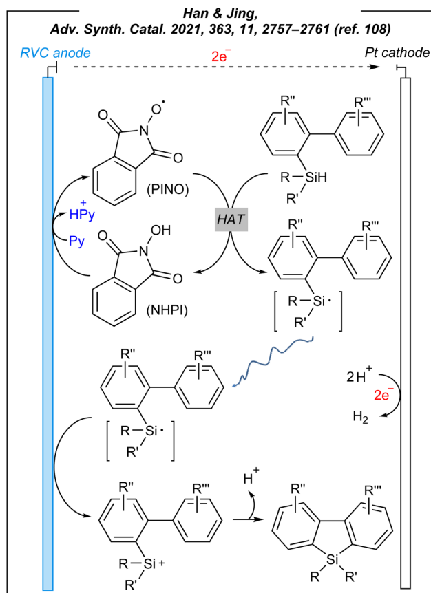
Fig. 13 Plausible mechanism for the electrocatalytic sila-Friedel-Crafts reaction.
