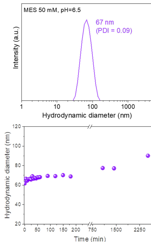
Fig. 6 DLS curve (top) and the evolution of the mean hydrodynamic diameter vs. time (bottom) for \text{Eu}(20\%):\text{NaBi}(\text{MoO}_4)_2@PAA NPs suspended in MES medium ( \text{pH} = 6.5 ). PDI values were < 0.1 in all cases.
