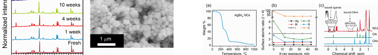
Fig. 6 (a) TGA data for a \text{AgBiI}_4 NC sample. (b) Changes in surface composition (atomic ratios normalized to \text{I} = 4 ) of \text{AgBiI}_4 film sample during XPS measurement of five consecutive cycles of spectra ( \text{Bi } 4f \rightarrow \text{I } 3d \rightarrow \text{Ag } 3d \rightarrow \text{O } 1s \rightarrow \text{C } 1s \rightarrow \text{N } 1s , duration of a cycle \sim 10 min). (c) ^1\text{H} NMR spectra of \text{AgBiI}_4 NCs, pure OA, and pure \text{OlAm} . The insets highlight the proton resonances related to bound ligands.
