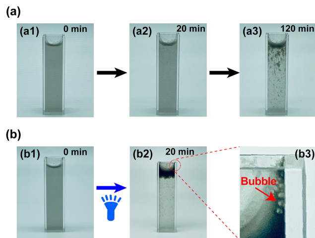
Fig. 4 Z-axis motion of PPy/ZIF-8 micromotors. (a) Slow self-floating of PPy/ZIF-8 micromotors (1.5 mg mL -1 ) under static conditions; (a1–a3) optical images illustrating the suspension state at 0, 20, and 120 min. (b) Incident blue light (0.6 W cm -2 ) from the bottom of the suspension to accelerate the Z-axis movement of PPy/ZIF-8 micromotors (1.5 mg mL -1 ); (b1 and b2) optical images illustrating the suspension state at 0 and 20 min during blue light irradiation; (b3) an enlarged image of (b2) showing the formation of bubbles.
