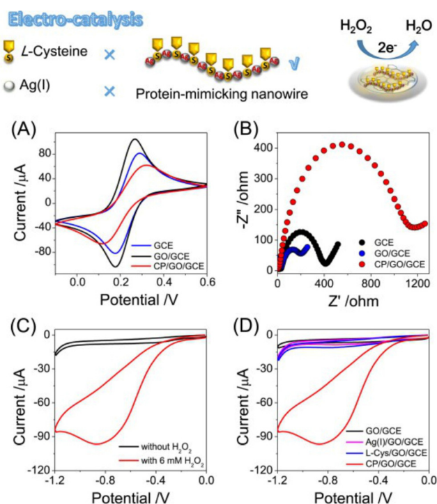
Fig. 5 (A) Cyclic voltammogram and (B) EIS of the bare GCE, GO/GCE and CP/GO/GCE in 5\ \text{mM}\ [\text{Fe}(\text{CN})_6]^{3-/4-} containing 0.1\ \text{M}\ \text{KCl} ; (C) cyclic voltammograms of CP/GO/GCE in the presence or absence of 6\ \text{mM}\ \text{H}_2\text{O}_2 ; (D) cyclic voltammograms of GCE, Ag(I)/GO/GCE, L-Cys/GO/GCE and CP/GO/GCE in 0.1\ \text{M}\ \text{PBS} (pH 7.0) containing 6\ \text{mM}\ \text{H}_2\text{O}_2 (reprinted from ref. 71 with permission from Elsevier).
