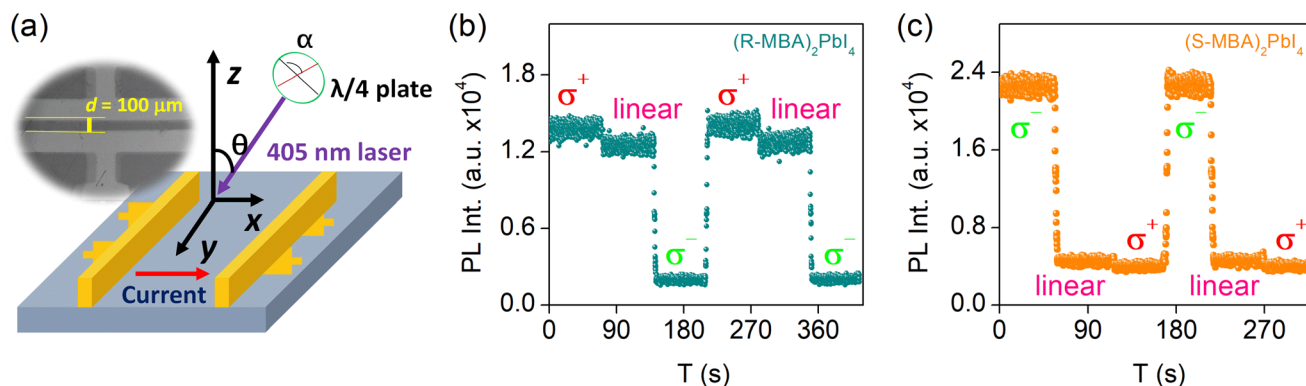
Fig. 2 (a) The schematic drawing of the lateral device configuration Au/chiral LHP/Au. The inset image shows the channel length of approximately 100 \mu m . (b) and (c) are the variations of the PL intensities due to the photo switches among the left-, linear and right-circularly polarized photoexcitation for (R-MBA)_2PbI_4 and (S-MBA)_2PbI_4 , respectively. The photoexcitation wavelength and the laser power were 405 nm and 90 mW, respectively.
