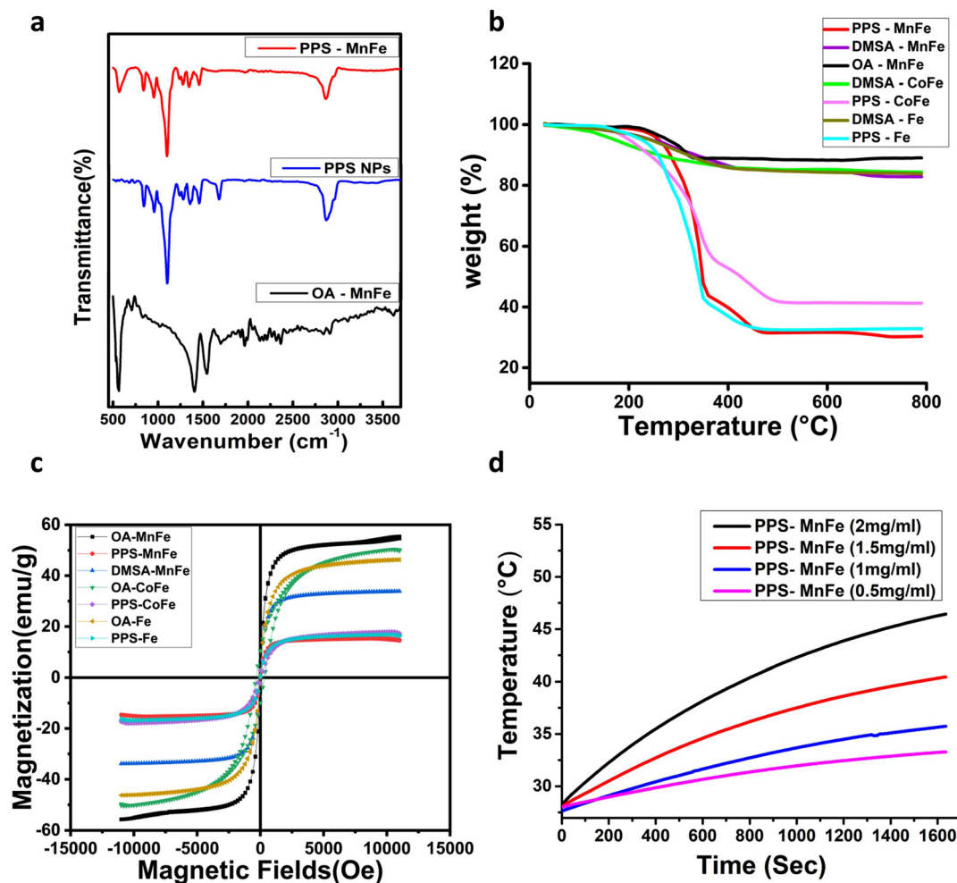
Fig. 3 Chemical and magnetic characterisation. (a) FTIR characterisation of plain MNPs (OA-MnFe), PPS NPs and PPS-MnFe NPs. Peaks attributed to MNPs at 500 cm -1 (Fe-O) are present in both the OA-MnFe and PPS-MnFe NPs graphs, and a peak at around 1100 (C-S) present in both the PPS NPs and PPS-MnFe NPs confirms the formation of NPs and PPS-MnFe. (b) Thermogravimetric analysis (TGA) graph presenting the % weight reduction during the melting of different coatings of OA, DMSA and PPS polymers. PPS-MNPs showed more % weight reduction compared with OA- and DMSA-coated MNPs. (c) Magnetization curve (magnetic hysteresis (M-H) loop) shows the saturation magnetization ( M_s ) of OA-MNPs, PPS-MNPs and DMSA-MnFe NPs. These curves show the superparamagnetic behaviours of NPs, which reduced in the case of PPS-MNPs. (d) Response of the PPS-MnFe NPs with varying concentrations (0.5–2 mg mL -1 ) to an external AMF using a 993 kHz frequency. This graph shows that the 2 mg mL -1 concentration is working better and can achieve a temperature rise from 28 °C in 46 °C in 25 min, wherein to attain a temperature rise from 37 °C to 42 °C, NPs took less than 10 min.
