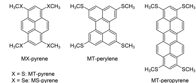
Fig. 1 Molecular structures of 1,3,6,8-tetrakis(methylthio)- and 1,3,6,8-tetrakis(methylseleno)-pyrene and (MT- and MS-pyrene), 2,5,8,11-tetrakis(methylthio)peropyrene (MT-ptylene), and 1,3,8,10-tetrakis(methylthio)peropyrene (MT-peropyrene).
