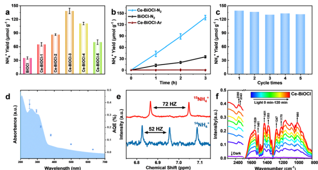
Fig. 2 Photocatalytic activity under a 300 W xenon lamp, ^{15}\text{N} isotope tracing results and in situ -FTIR results. (a) Photocatalytic \text{NH}_4^+ yields of BiOCl, Ce-BiOCl-1, Ce-BiOCl-2, Ce-BiOCl-3, Ce-BiOCl-4, and Ce-BiOCl-5. (b) Photocatalytic \text{NH}_4^+ yields for 3 h under Ar and \text{N}_2 atmospheres. (c) Cycling stability in the first three hours for the cycling stability test of Ce-BiOCl. (d) AQE of Ce-BiOCl. (e) ^1\text{H} NMR spectra of ^{15}\text{NH}_4^+ and ^{14}\text{NH}_4^+ products after photocatalytic reactions using ^{15}\text{N}_2 and ^{15}\text{N}_2 gases as the nitrogen source, respectively. (f) The in situ -DRIFTS of Ce-BiOCl under illumination.
